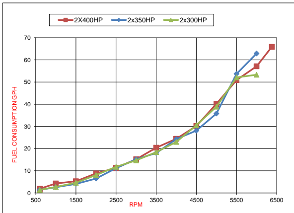
Fuel Consumption
