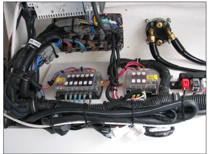
Fuse Panels Located Behind Helm
