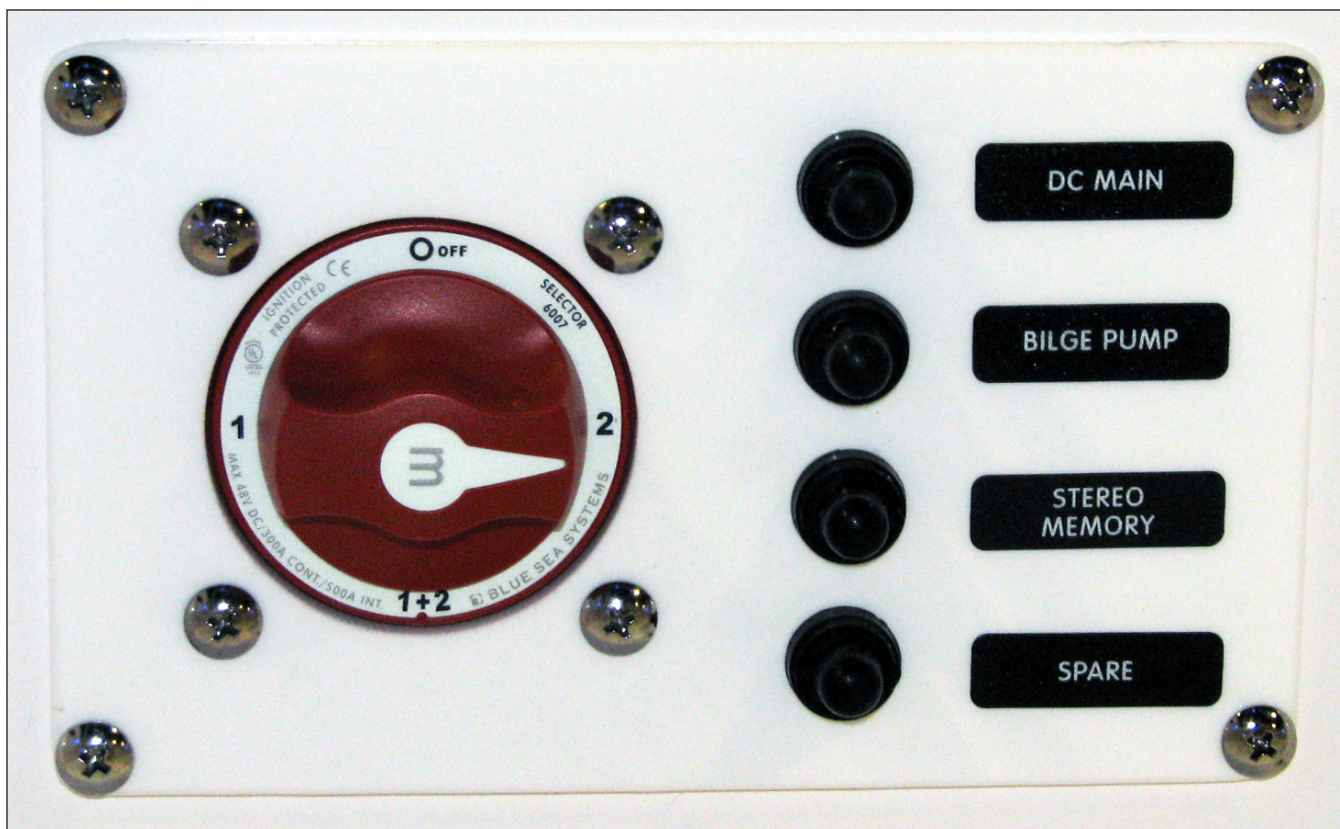
Battery Selector Switch and Circuit Breakers
