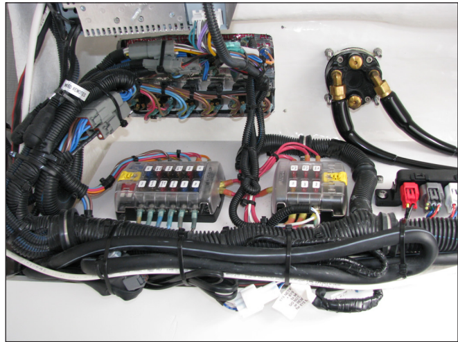
Helm Components and Fuse Panels
