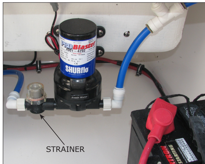
Typical Fresh Water Pump and Strainer
