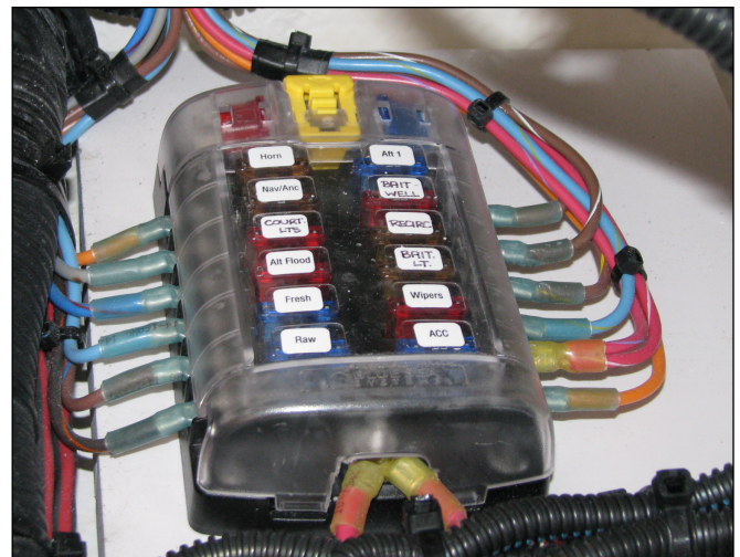
Accessory Fuse Panel Behind Helm
