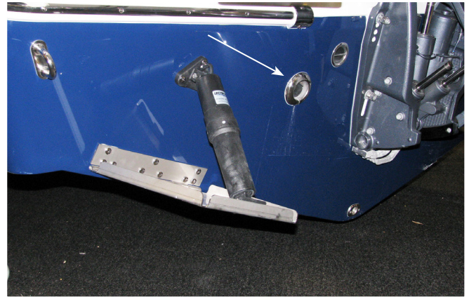
Transom Scupper Drain Check Valve Assembly
