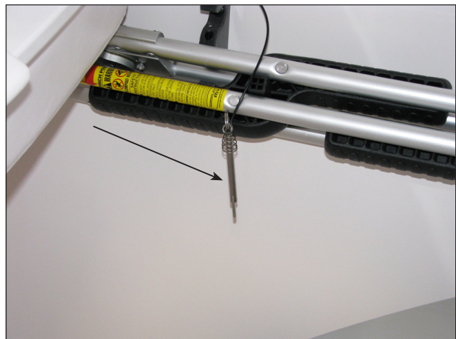
Forward Boarding Ladder Folded in Storage Bracket Storage Bracket Quick Release Pin
