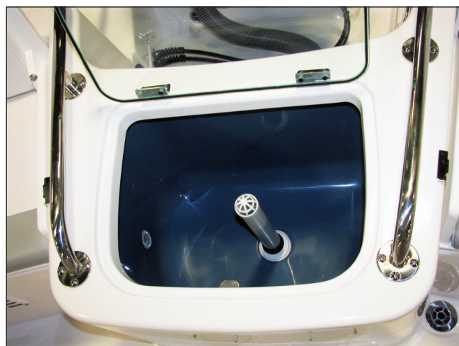
Baitwell and Overflow Tube
