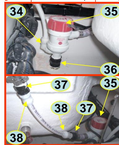
Livewell Pump
