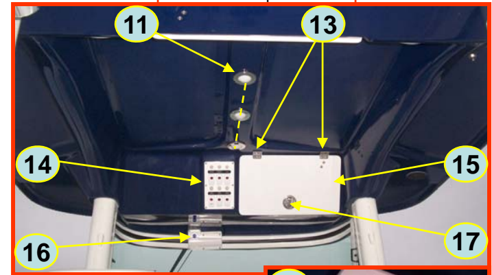
Nav Light
