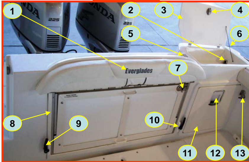
Transom Interior
