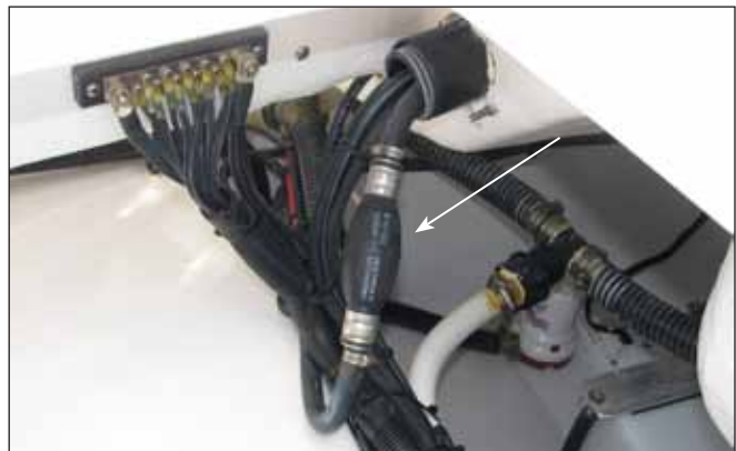
Primer Bulb Below Starboard Sterns Seat
